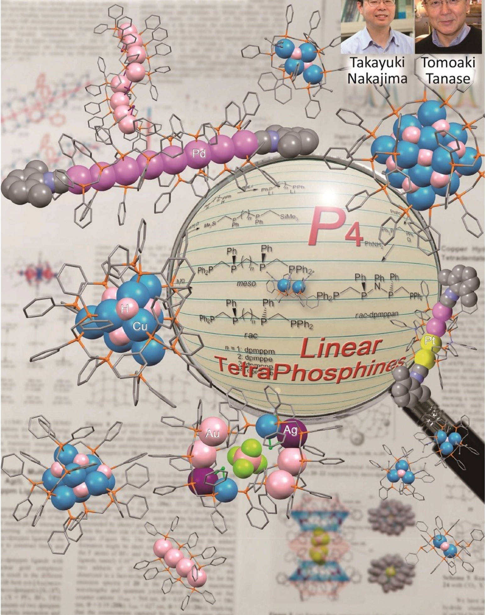
Figure 1. (a) Four-fold arrangement of two P_4 ligands.
